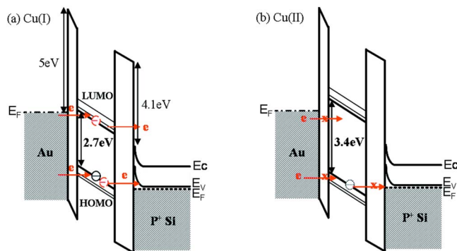
FIG. 4. (Color online) Band diagram of the molecular rotor device under negative bias at (a) high conductivity state of Cu(I) system and (b) low conductivity state of Cu(II) system. As oxidation happens, one electron in the valence band tunnels out of the molecular layer and the energy states move down. The band gap increases so that the conduction path for electrons is closed, resulting in NDR.
