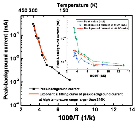
FIG. 3. (Color online) Arrhenius plot of the peak minus background current. The activation energy of rotation was extracted to be 0.3 eV by exponentially fitting the curve of the measurement data higher than 244 K. The inset shows the peak current as well as the background current at 0.5 V and -0.5 \text{ V} , respectively. The weak temperature dependence of the background current implies tunneling transport of electrons.
