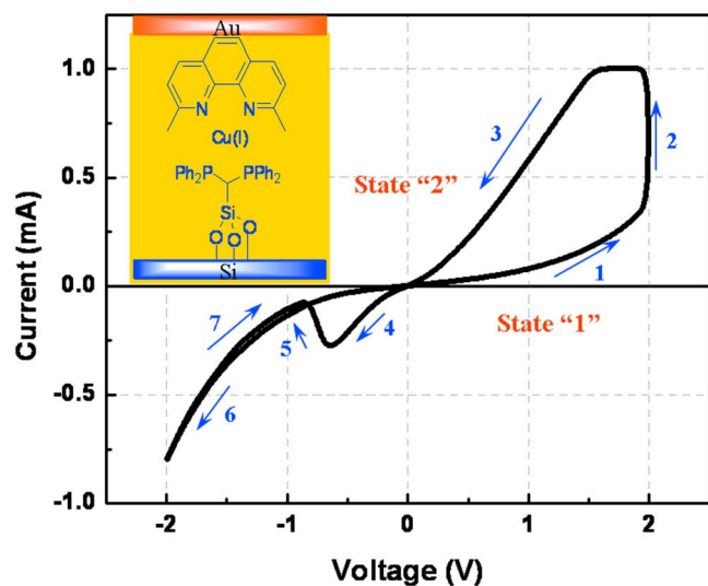
FIG. 2. (Color online) I - V characteristics of the monolayer device with the bisP stator. State “1” represents the low conductivity state, while state “2” is the high conductivity state. The turning voltage between state “1” and state “2” is determined by the redox energy of the copper system. The difference in value of the turning voltage between positive and negative ranges is due to the different contact energy barriers of the two electrodes. The arrows show the sequence of the voltage scan. Arrows “4” and “5” correspond to the band diagrams in Figs. 4(a) and 4(b), respectively (to be discussed later).
