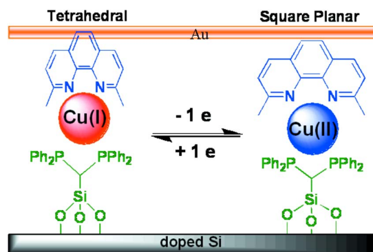
FIG. 1. (Color online) The schematic structure of the molecular rotor device composed of a bisP stator, a copper metal axle, and a diimine rotator. The diimine ligand on top, 2,9-dimethyl-1,10-phenanthroline, rotates upon reduction and oxidation in the direction as illustrated with arrows.
